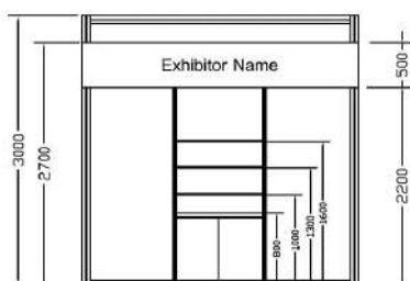
FRONT VIEW Scale 1:50
