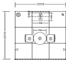
TOP VIEW Scale 1:50
